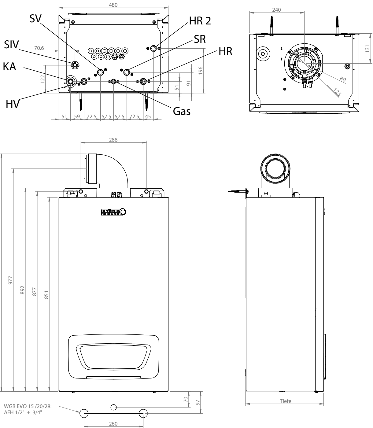
Abb. 9: WGB EVO 15–38 i
